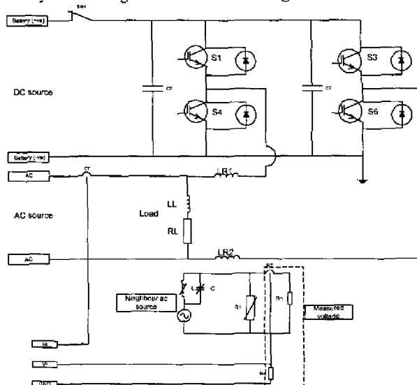
Figure 1 -- System Configuration
