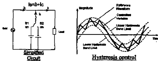
Figure 2. Control Strategy of the power converter
